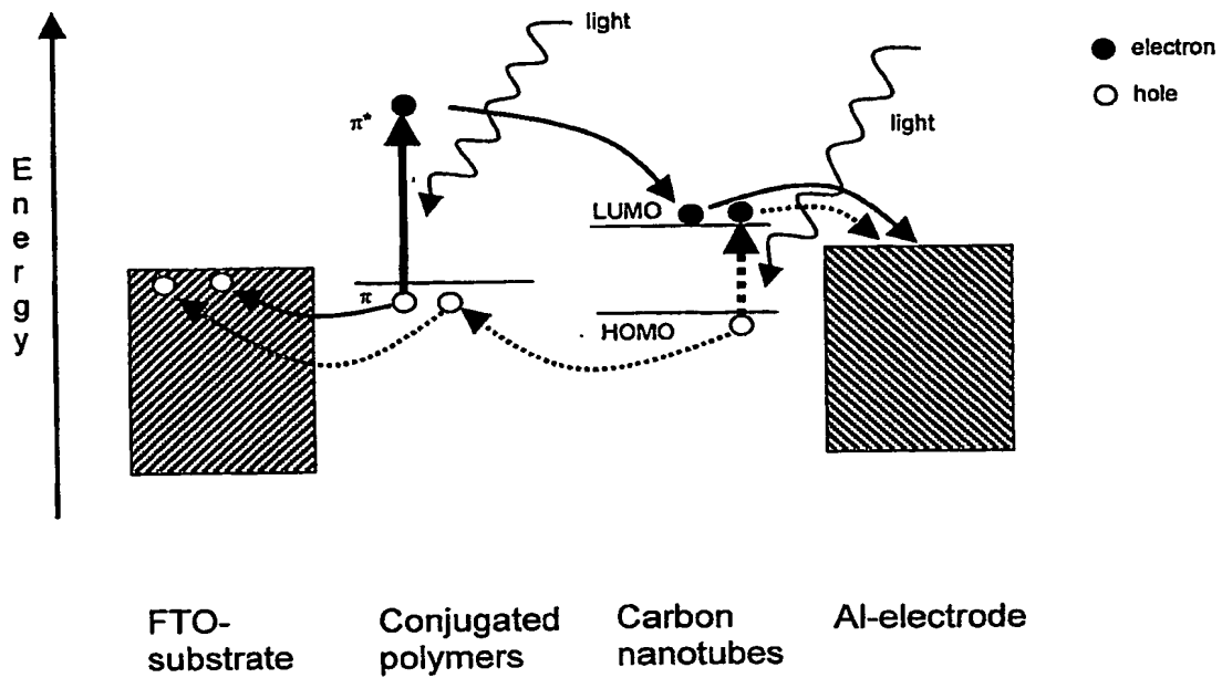
Fig. 2: Schematic band diagram and different excitation processes of and in a carbon nanotube based photovoltaic device according to the present invention.
